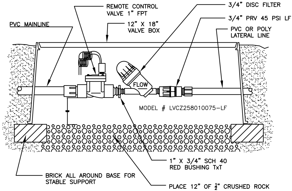
LOW VOLUME (LOW FLOW) CONTROL SYSTEM(.25 GPM-4.4 GPM)
