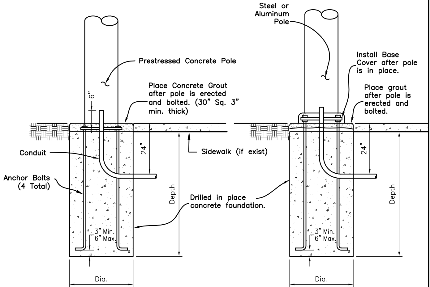
Foundation Dimensions
