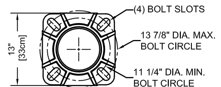
ANCHOR PLATE DETAIL
