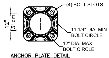
ANCHOR PLATE DETAIL
