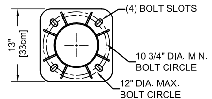
ANCHOR PLATE DETAIL
