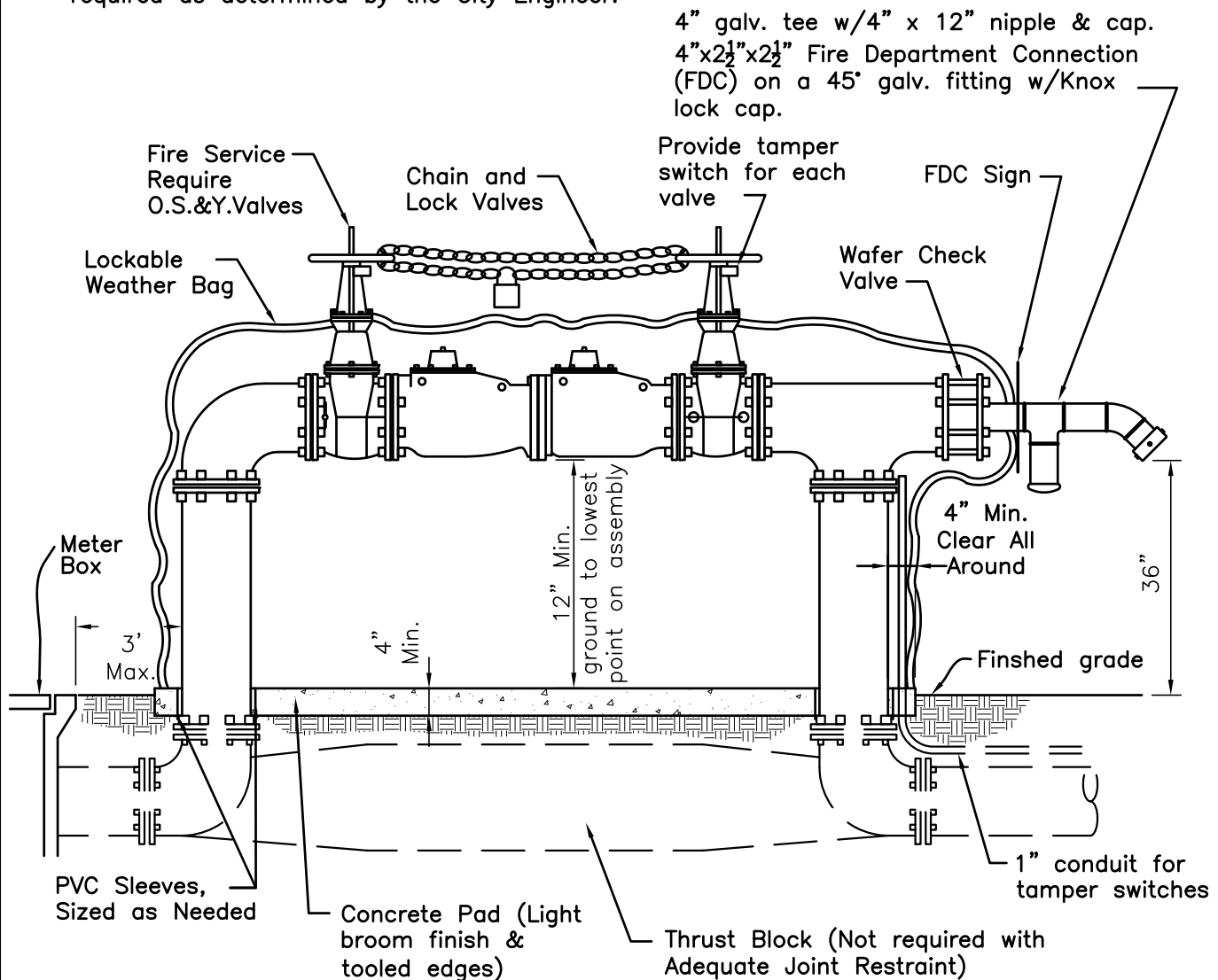
TYPICAL SIDE VIEW
