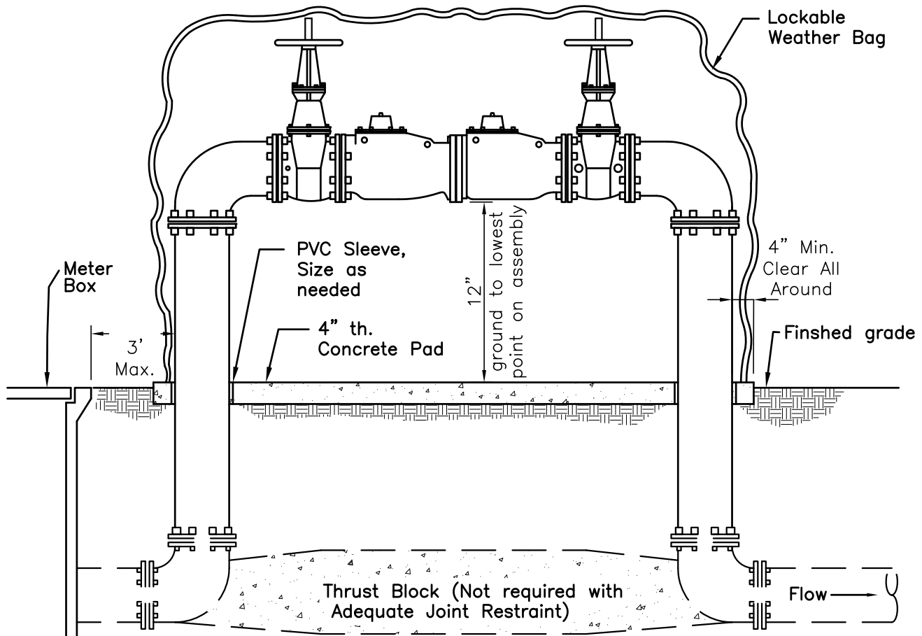
TYPICAL SIDE VIEW
