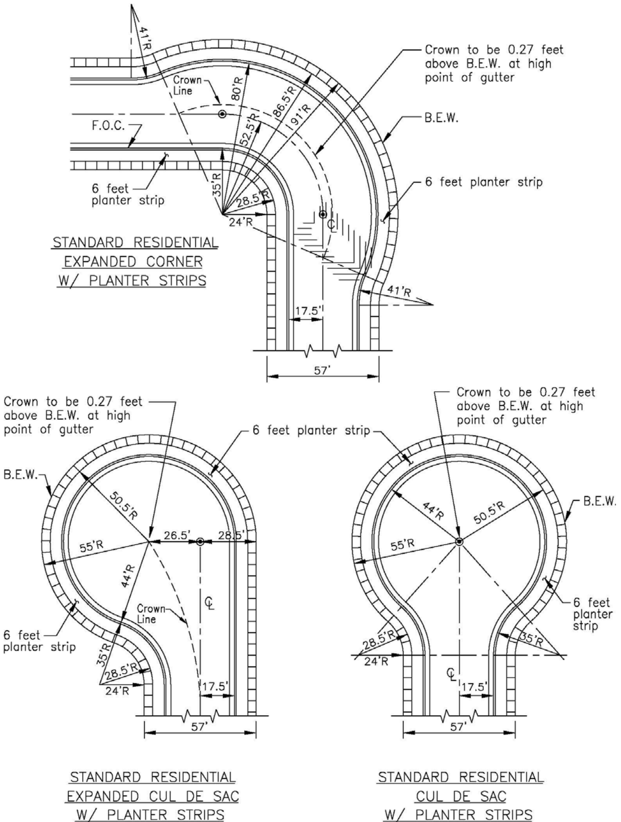
3.28 FIGURE 3A – GEOMETRICS OF EXPANDED CORNERS AND CUL-DE-SACS
