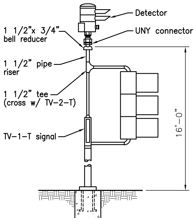
I-B MOUNTING LOCATION
