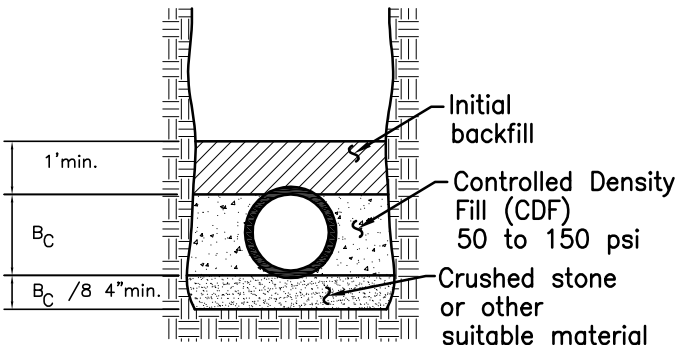
Load Factor 2.8
