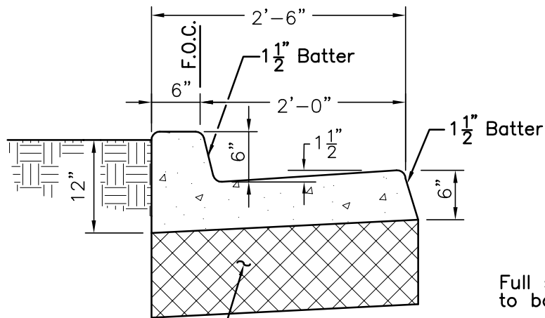
Full Street Section Cl. 2 A.B.
