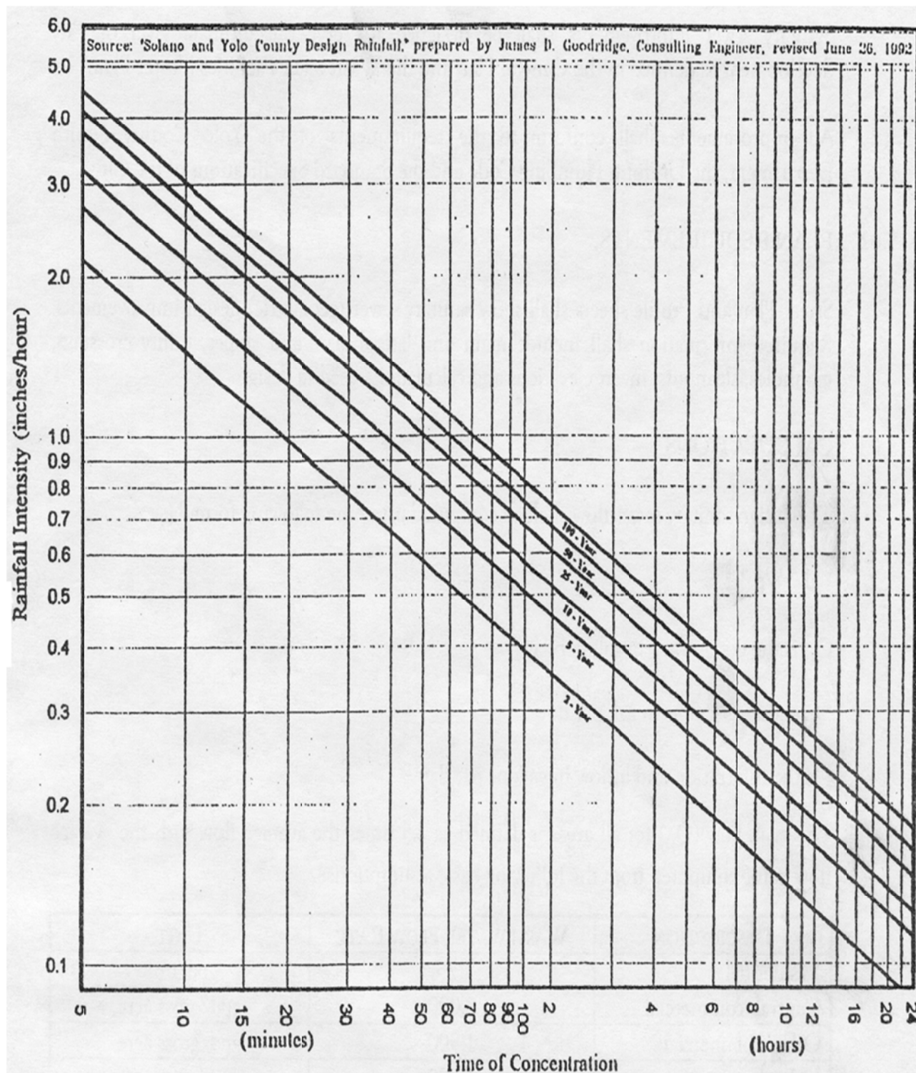
4.39 FIGURE 4N – RAINFALL INTENSITY DURATION FREQUENCY
