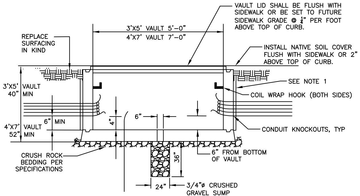
ELEVATION VIEW
