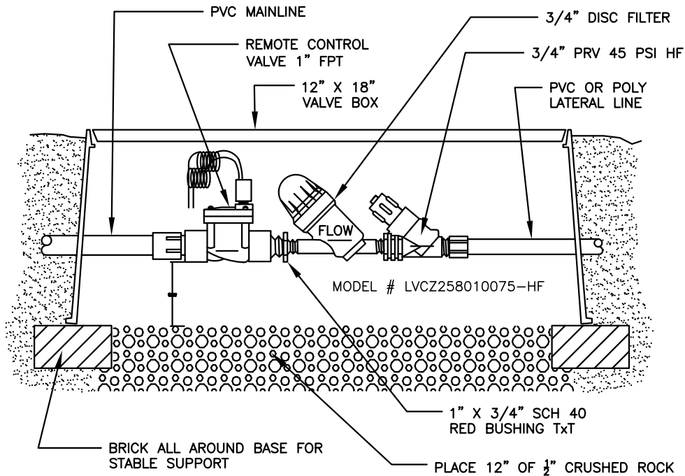
LOW VOLUME (HIGH FLOW) CONTROL SYSTEM(4.5 GPM-17.6 GPM)
