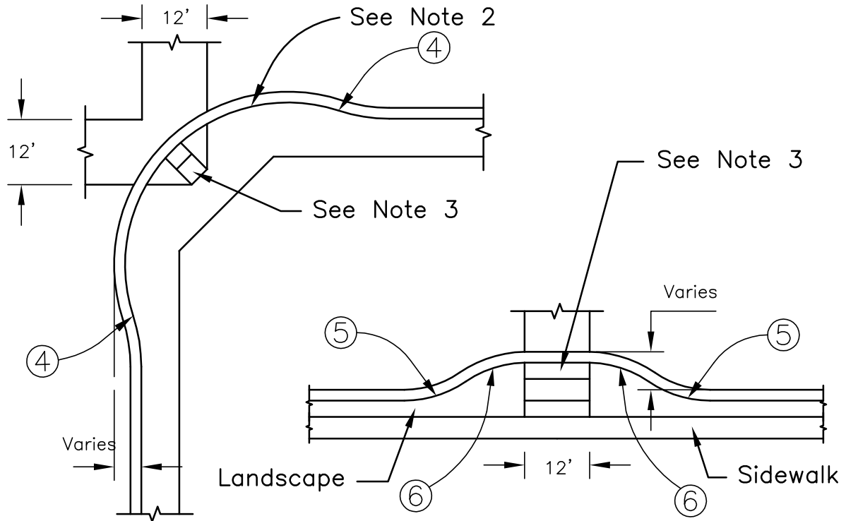
CURB BULB-OUT DETAIL AT END OF BLOCK
