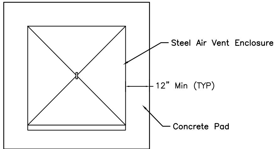
Concrete Pad Plan
