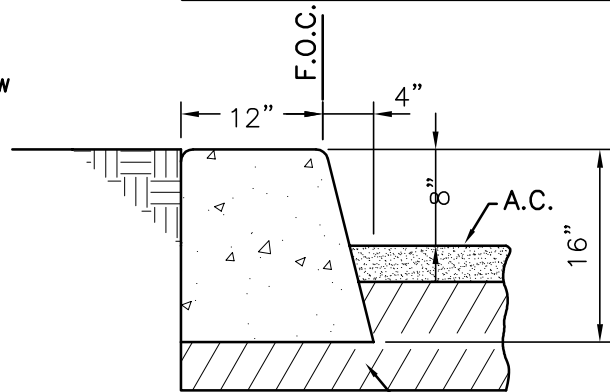
Full Street Section
