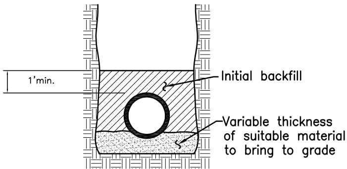
Load Factor 1.1 Flat or Restored Trench Bottom
