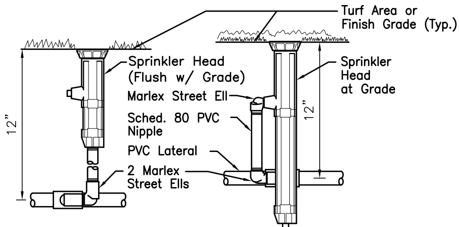
6" HIGH POP-UP
