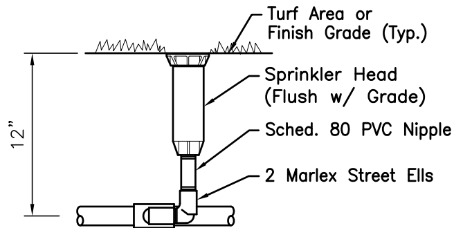
4" HIGH POP-UP
