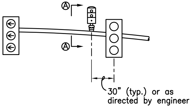
WITH LEFT TURN POCKET
