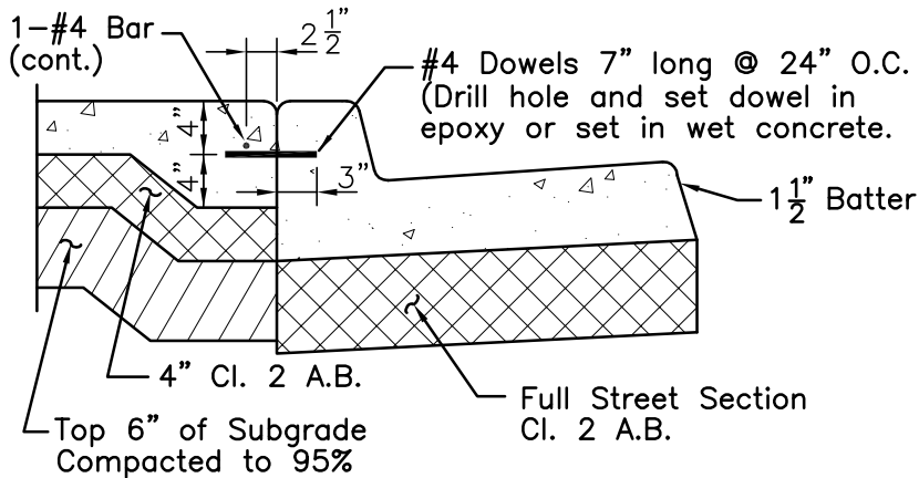
Full Street Section Cl. 2 A.B.
